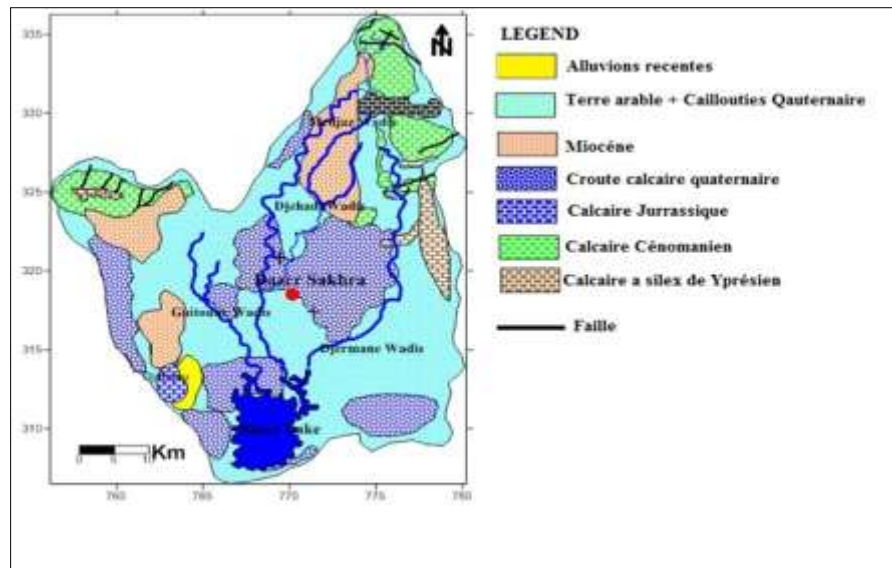
Fig. 2 Geological map of the studied area
