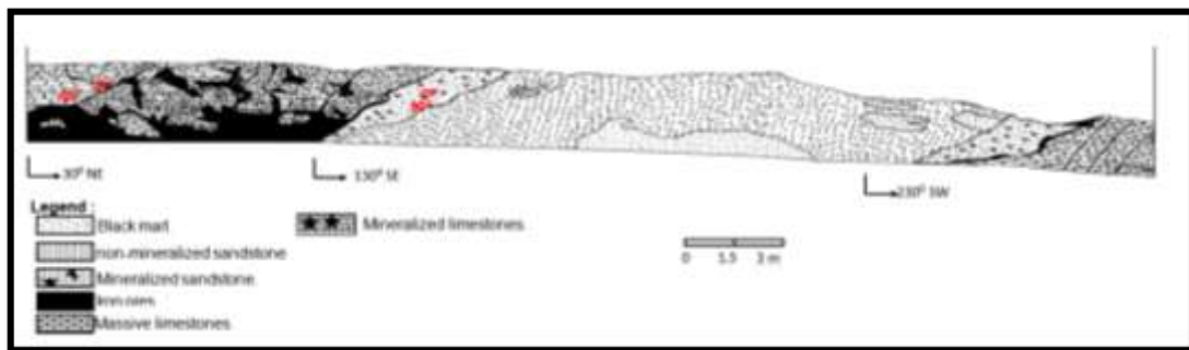
Figure 2. Geology career front bench N° :1020m.
