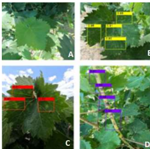
Figure 12. The process of applying the deep learning model A: healthy plant, B: powdery mildew ( Uncinula necator Schw., Burr.), C: mildew ( Plasmopara viticola Berk. Et. Curt, Berl et de Toni), D: Phomopsis cane and leaf spot ( Phomopsis viticola Sacc.) (Altaş et al., 2023).
