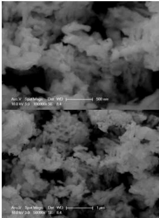
Figure 3. SEM images (left) x100000 and (right) x50000 of \text{Nd}_2\text{O}_3 specimen.
