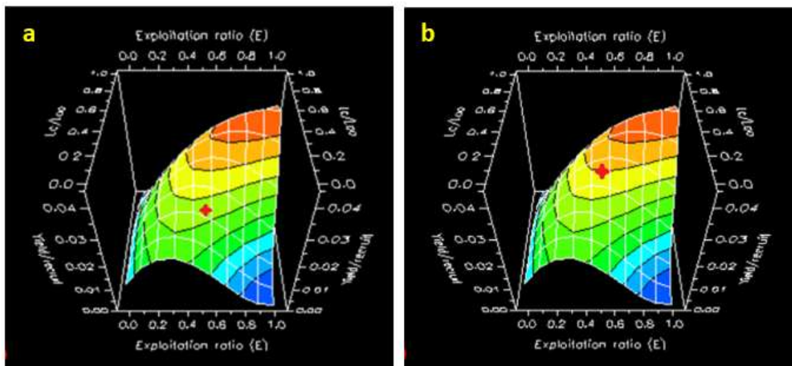
Figure 3. Relative Yield per Recruit Analysis (Knife-edge Selection) for the Ohrid trout stock as a function of the exploitation rate (E) and the ratio of length at first capture to asymptotic length ( L_c/L_{\infty} ) (a) Y'/R of the stock (indicated by the red star on the isobars) for E=0.51 \text{ yr}^{-1} and L_c=20.4 \text{ cm} . (b) Y'/R of the stock (indicated by the red star on the isobars) for E=0.51 \text{ yr}^{-1} and L_c=32.0 \text{ cm} .
